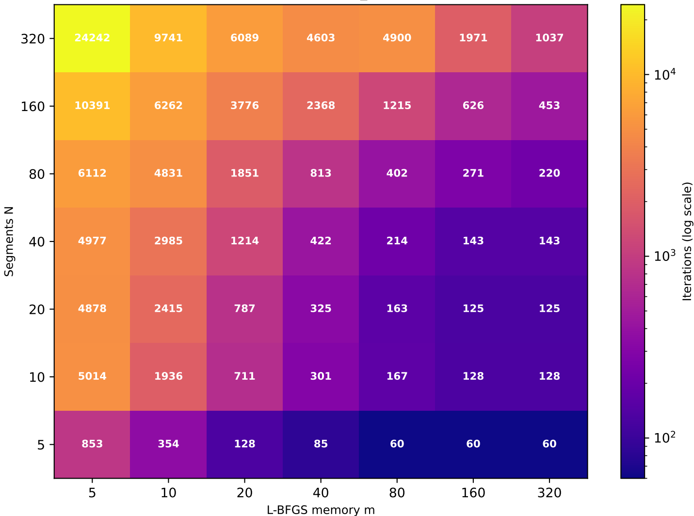
Recurrence T \approx 5.23 (target T=5 , rec_id=60) [49/49 converged]
