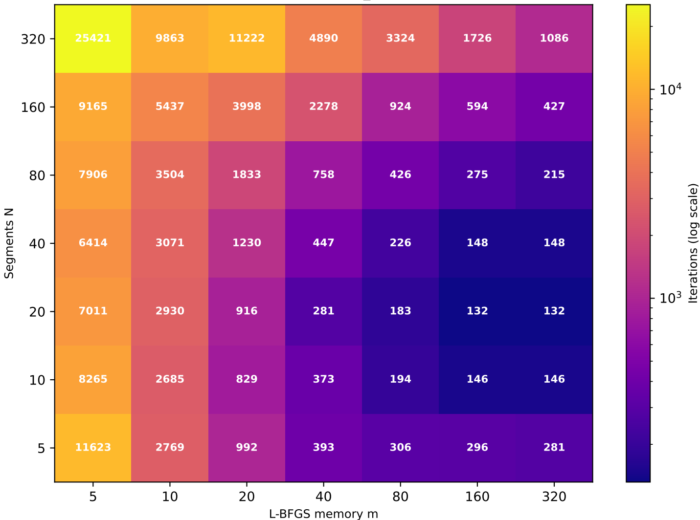
Recurrence T \approx 5.78 (target T=5 , rec_id=67) [49/49 converged]
