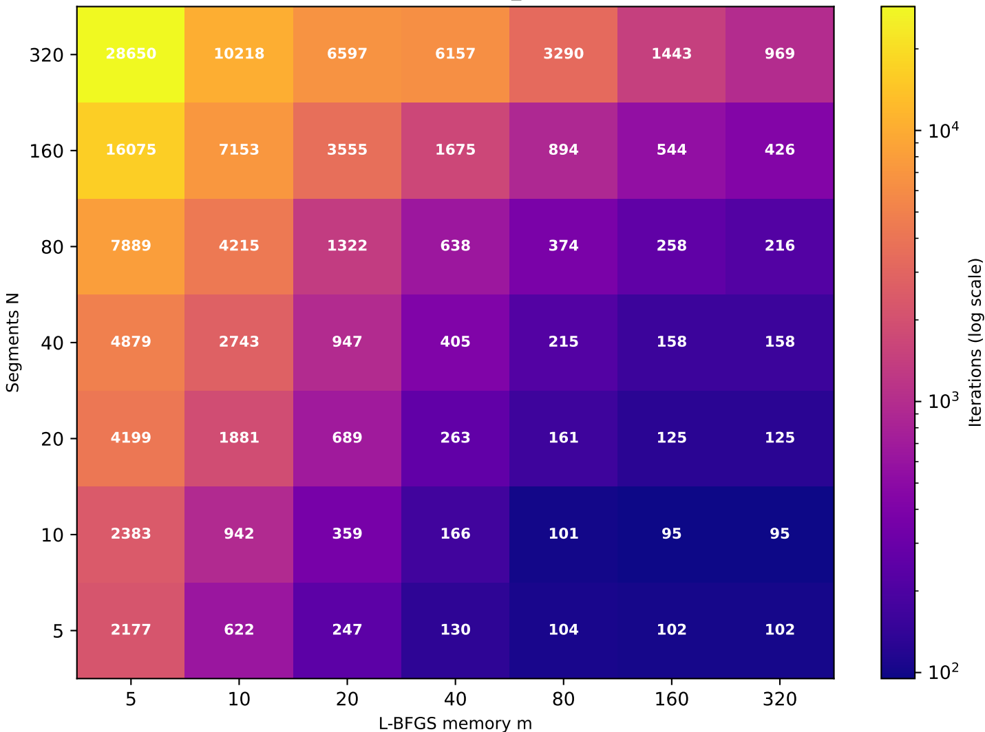
Recurrence T \approx 4.42 (target T=5 , rec_id=69) [49/49 converged]
