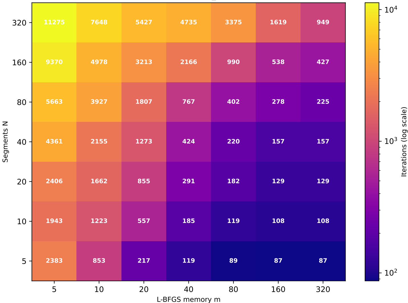
Recurrence T \approx 4.59 (target T=5 , rec_id=71) [49/49 converged]
