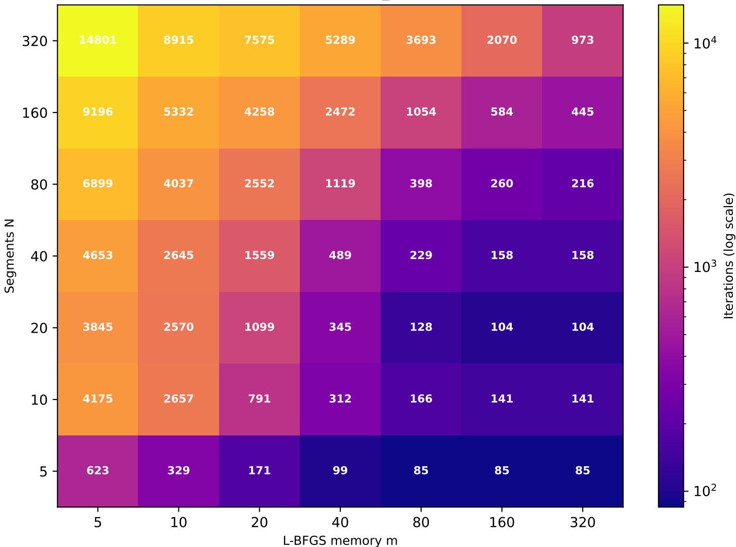
Recurrence T \approx 5.37 (target T=5 , rec_id=72) [49/49 converged]
