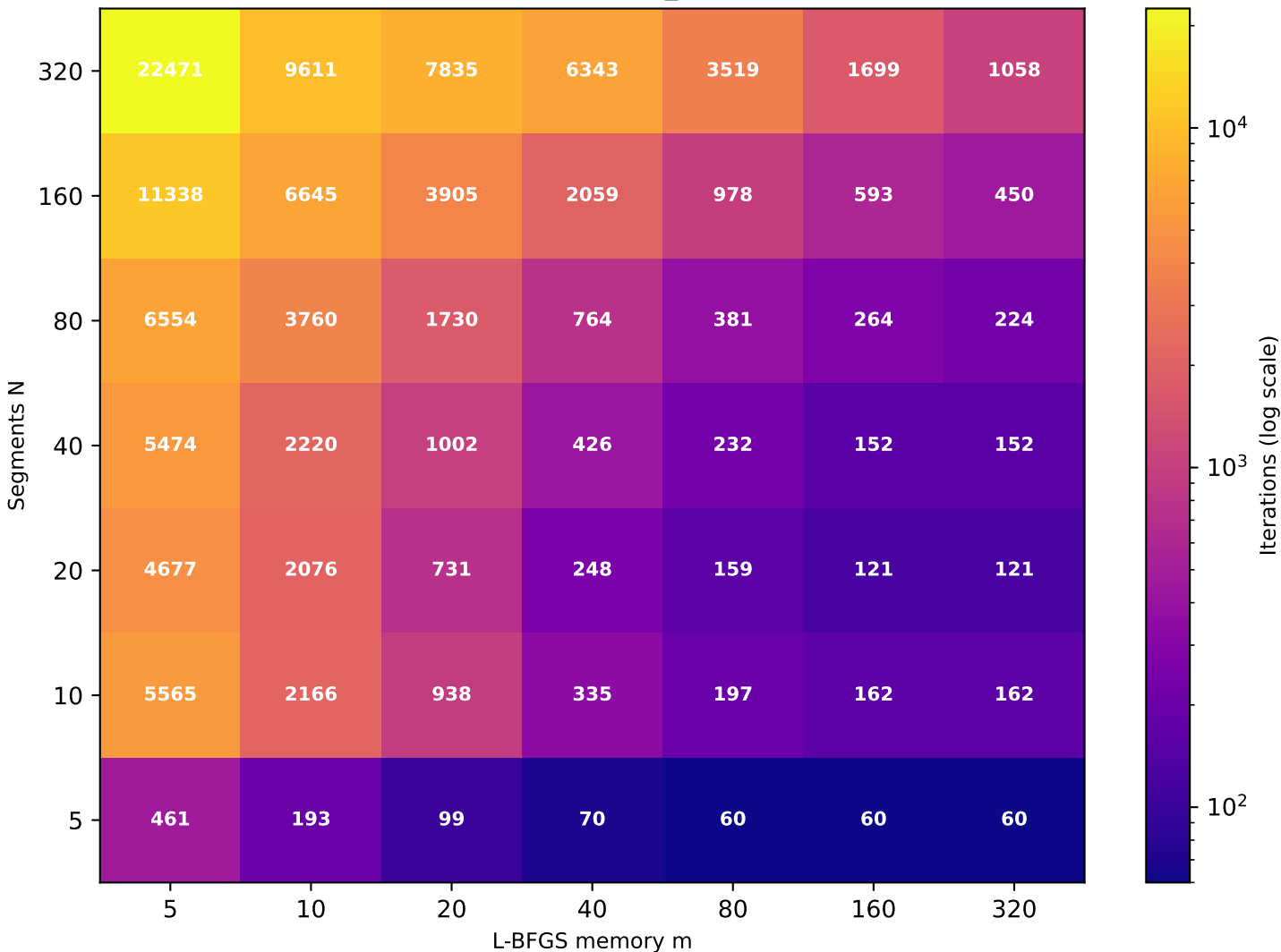
Recurrence T \approx 5.10 (target T=5 , rec_id=74) [49/49 converged]
