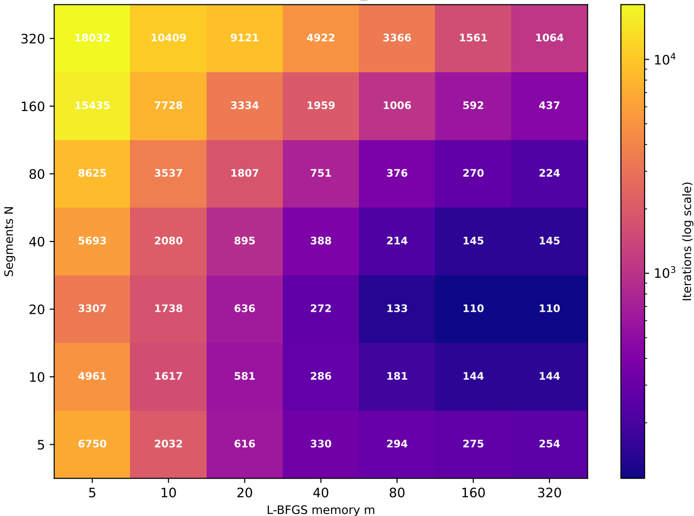
Recurrence T \approx 5.10 (target T=5 , rec_id=76) [49/49 converged]
