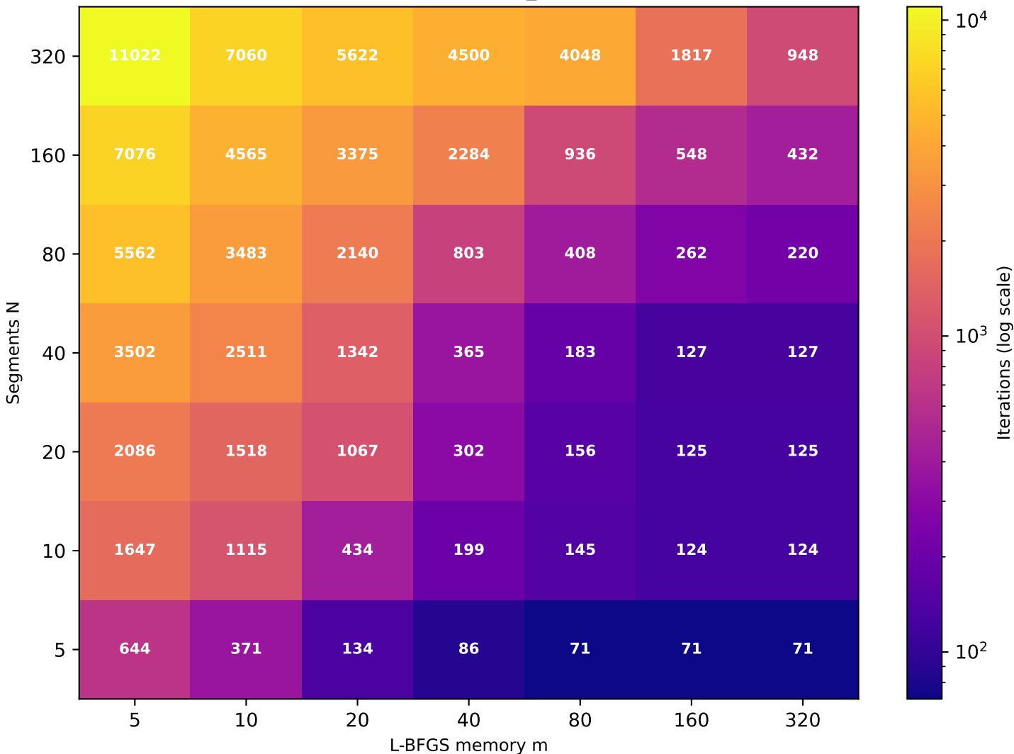
Recurrence T \approx 4.61 (target T=5 , rec_id=77) [49/49 converged]
