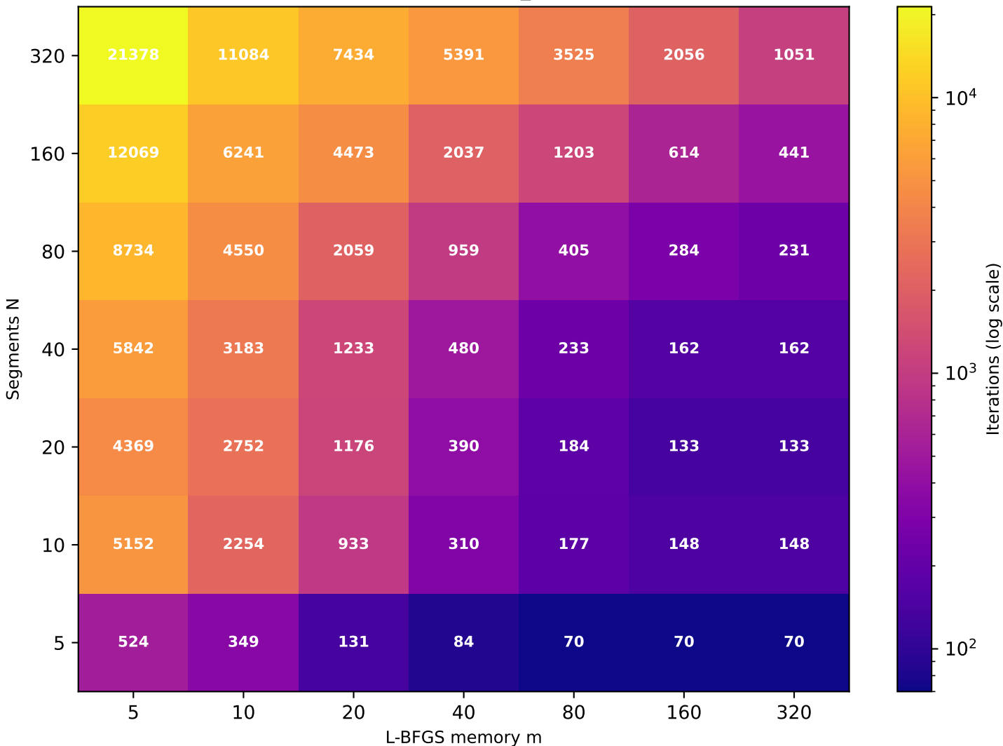
Recurrence T \approx 6.00 (target T=5 , rec_id=79) [49/49 converged]
