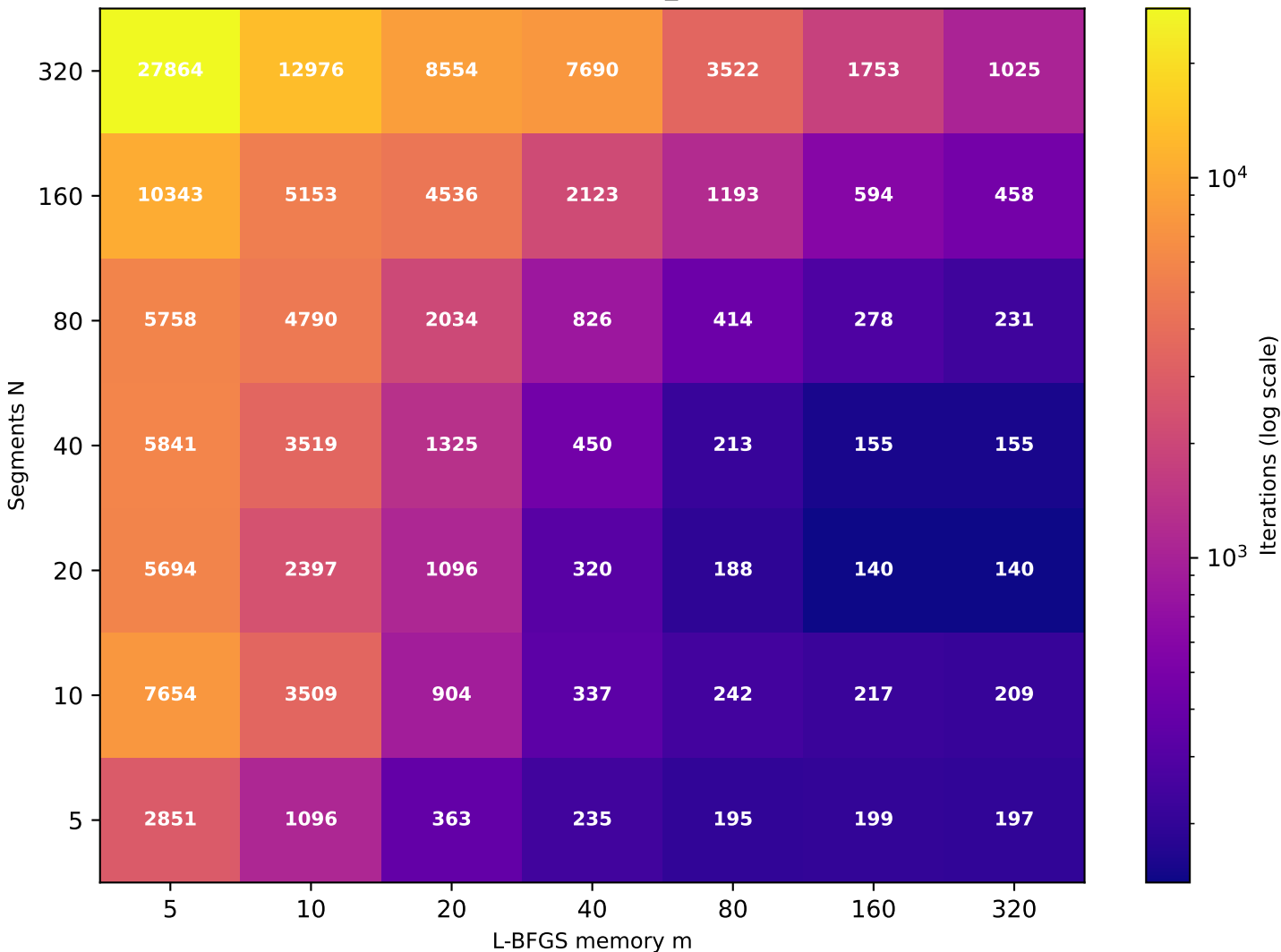
Recurrence T \approx 5.23 (target T=5 , rec_id=83) [49/49 converged]
