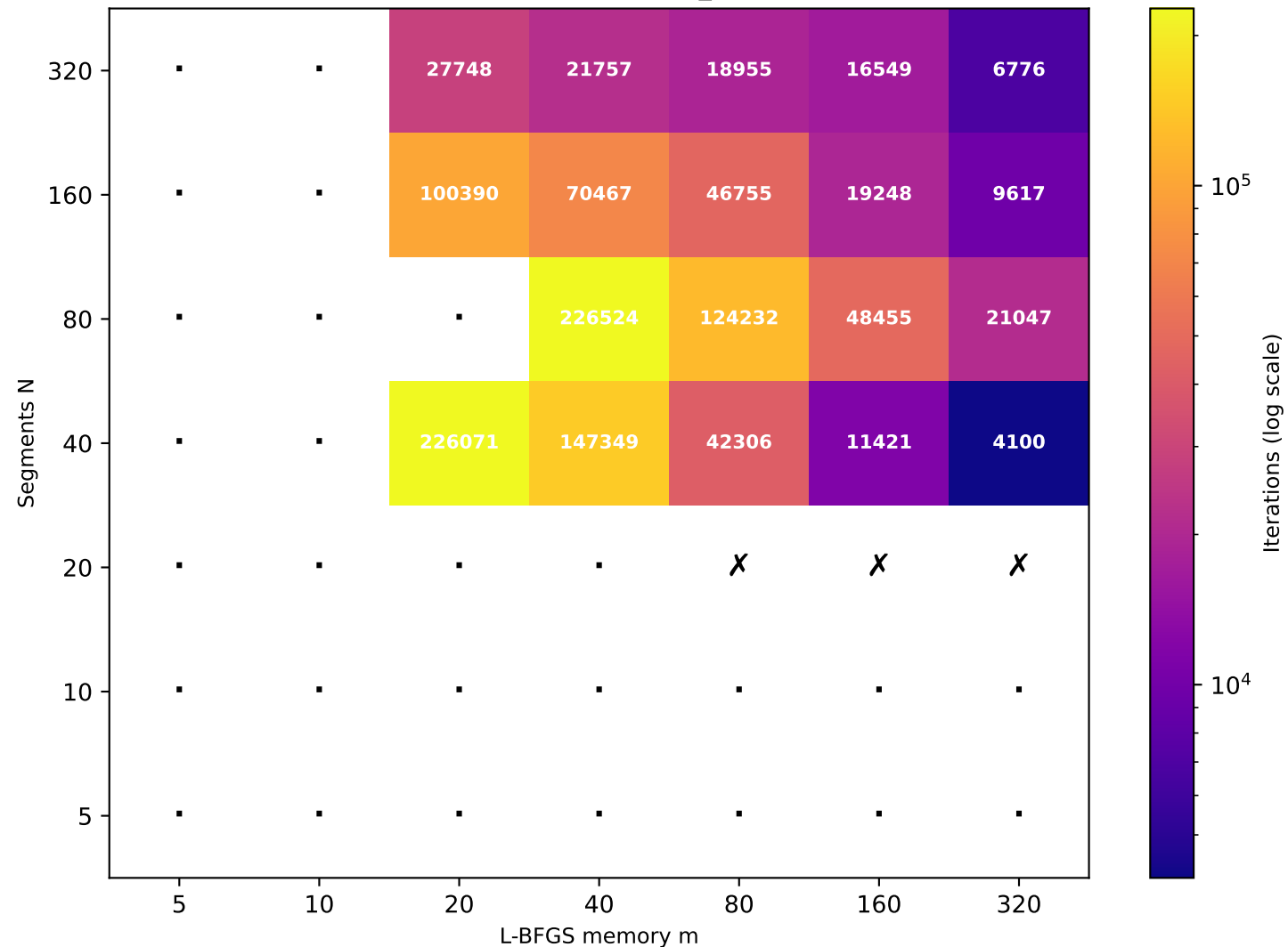
Recurrence T \approx 80.09 (target T=80 , rec_id=3) [19/49 converged]
