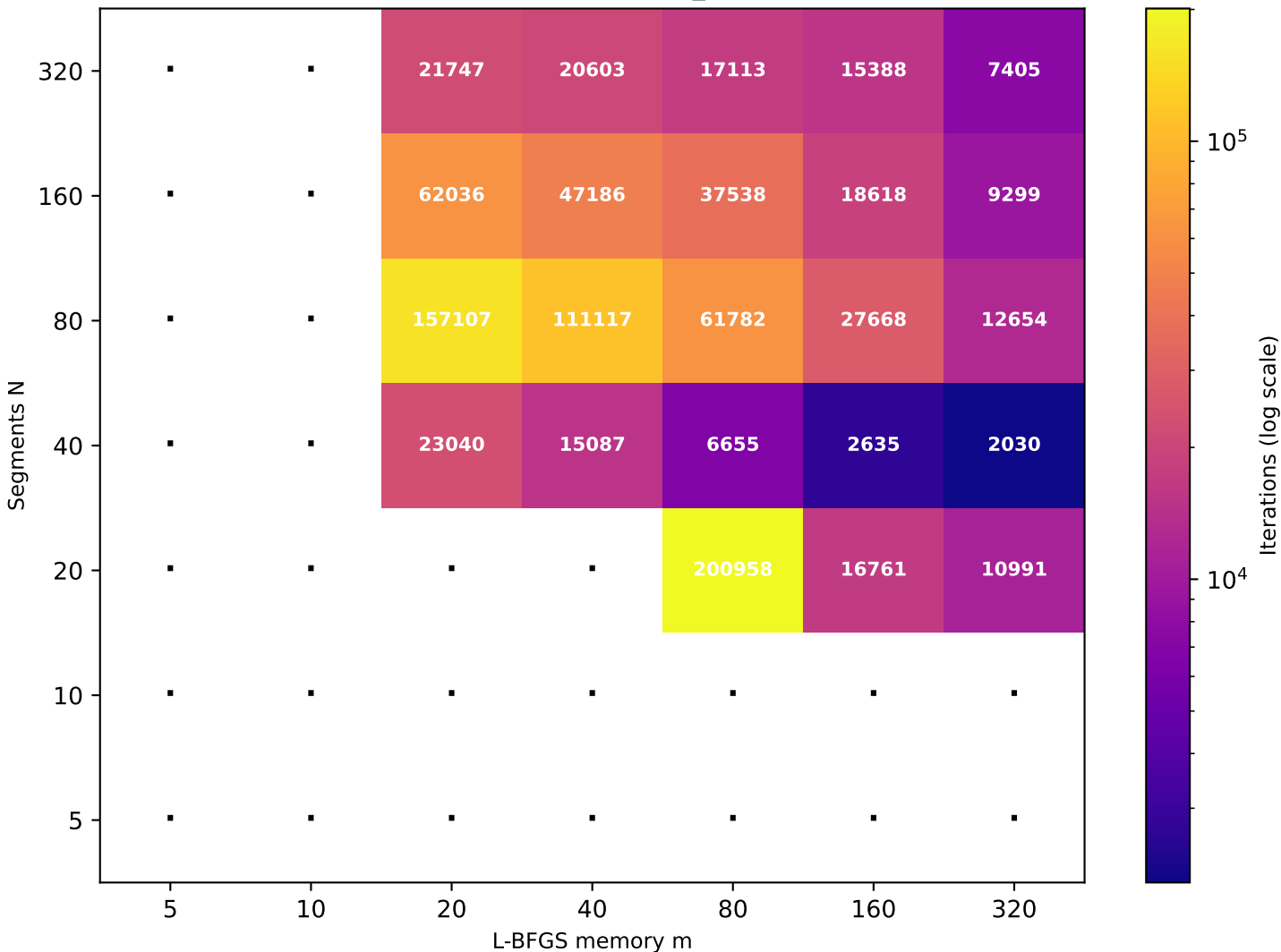
Recurrence T \approx 80.51 (target T=80 , rec_id=4) [23/49 converged]
