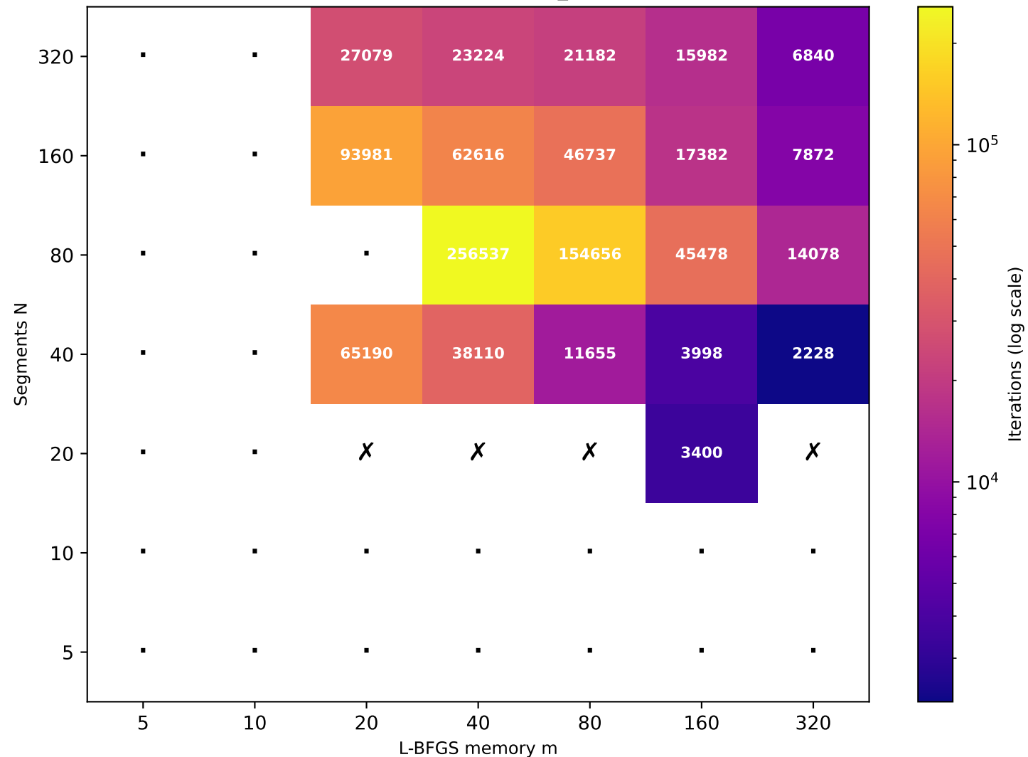
Recurrence T \approx 80.32 (target T=80 , rec_id=5) [20/49 converged]
