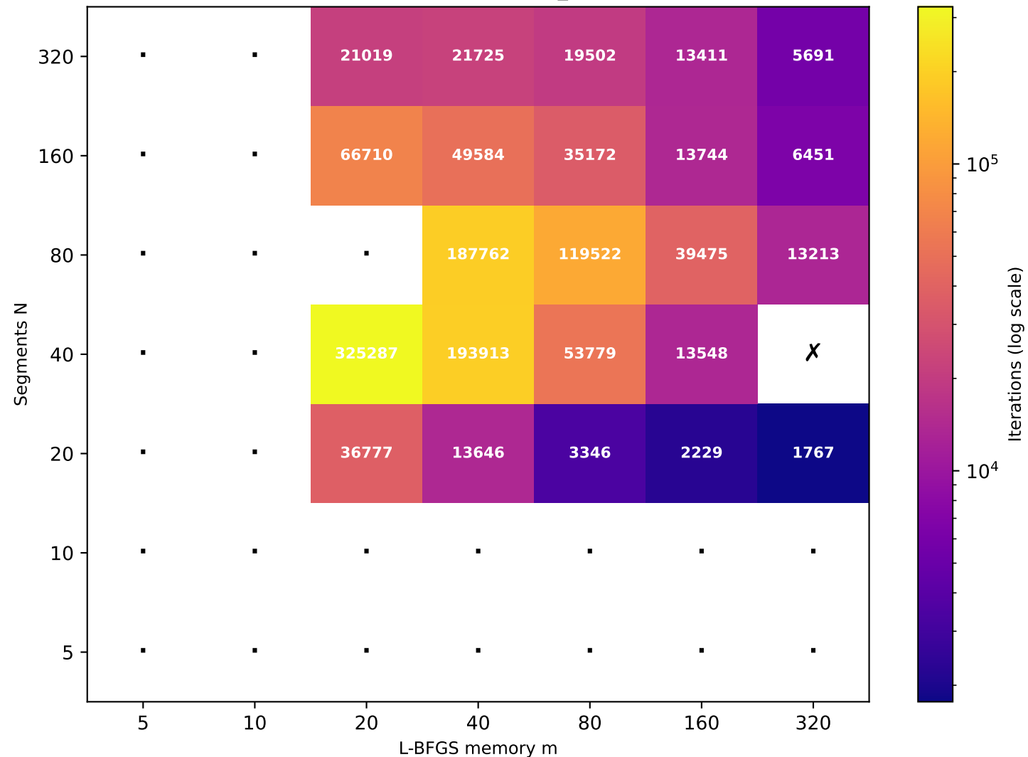
Recurrence T \approx 78.15 (target T=80 , rec_id=8) [23/49 converged]
