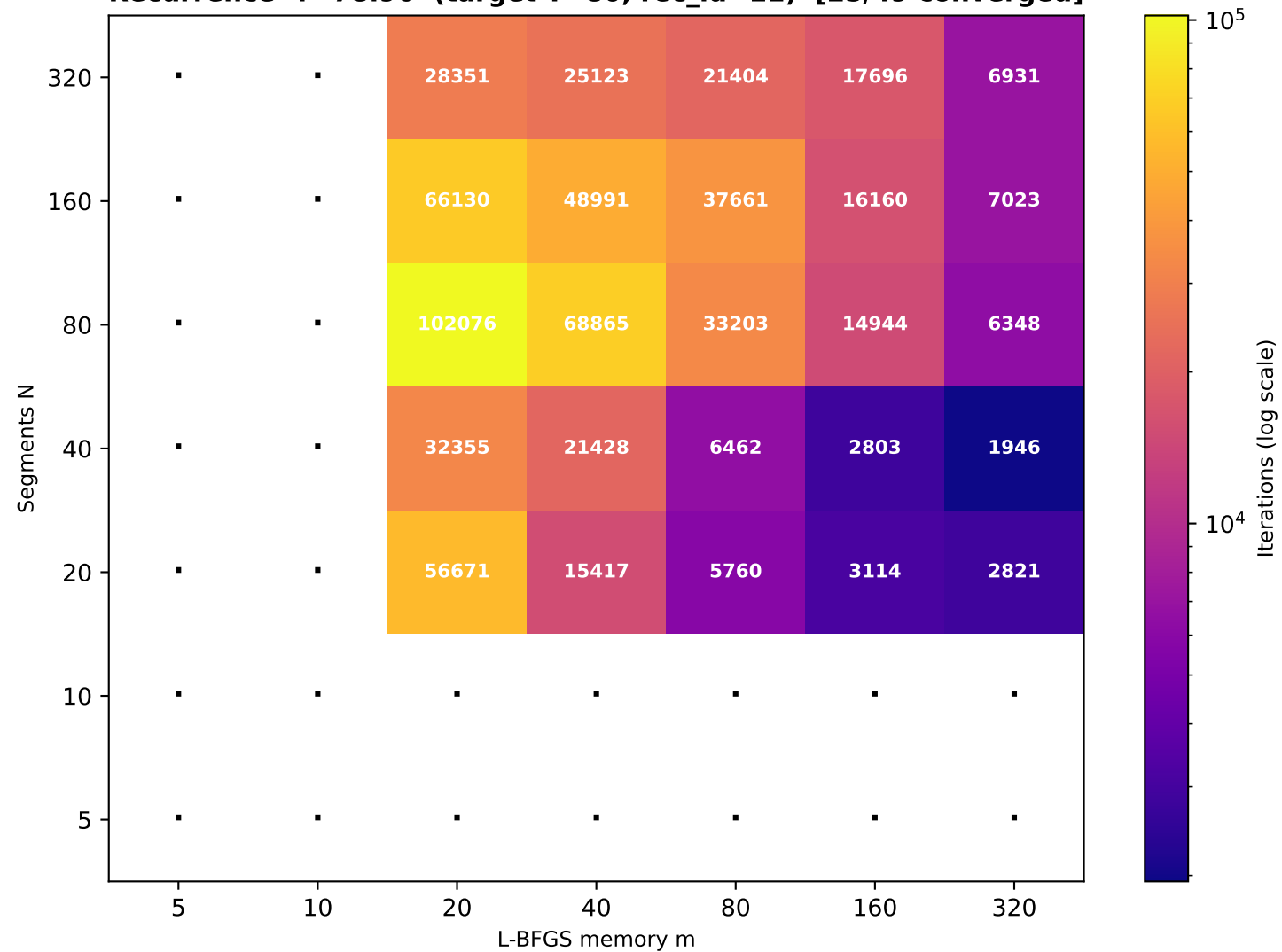
Recurrence T \approx 78.96 (target T=80 , rec_id=11) [25/49 converged]
