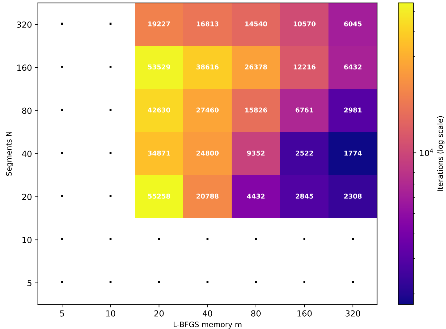
Recurrence T \approx 78.67 (target T=80 , rec_id=12) [25/49 converged]
