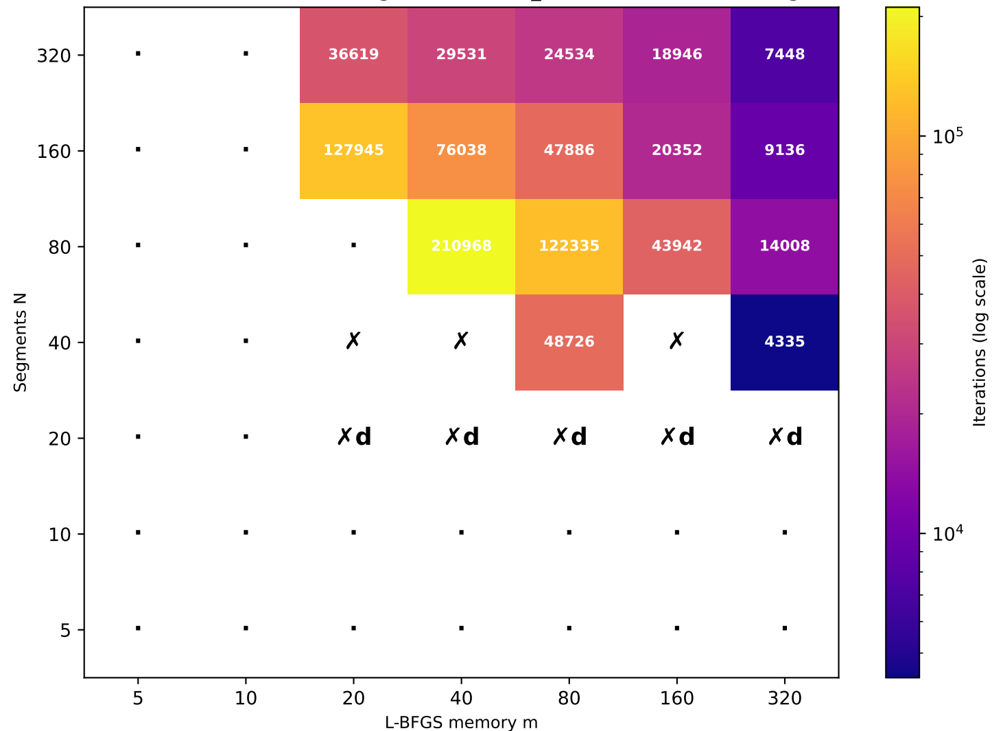
Recurrence T \approx 81.05 (target T=80 , rec_id=13) [16/49 converged]
