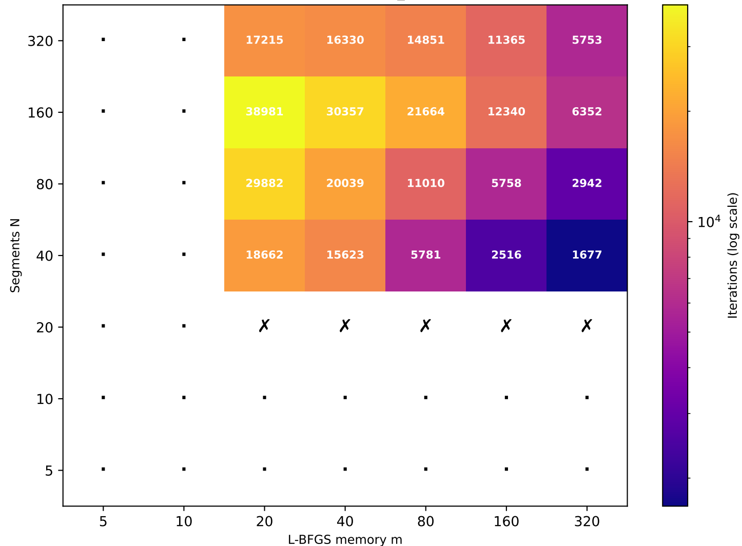
Recurrence T \approx 81.58 (target T=80 , rec_id=14) [20/49 converged]
