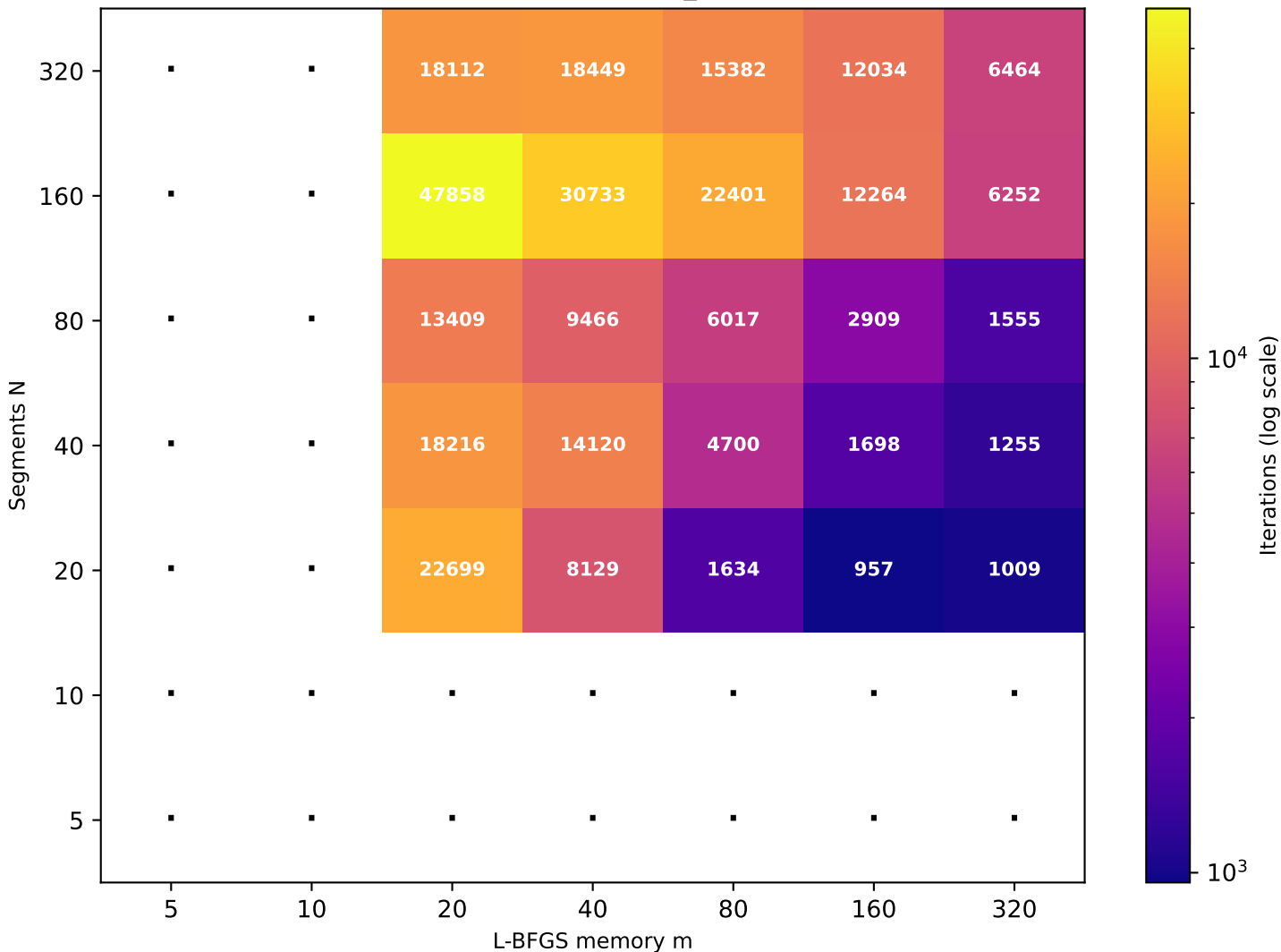
Recurrence T \approx 78.78 (target T=80 , rec_id=17) [25/49 converged]
