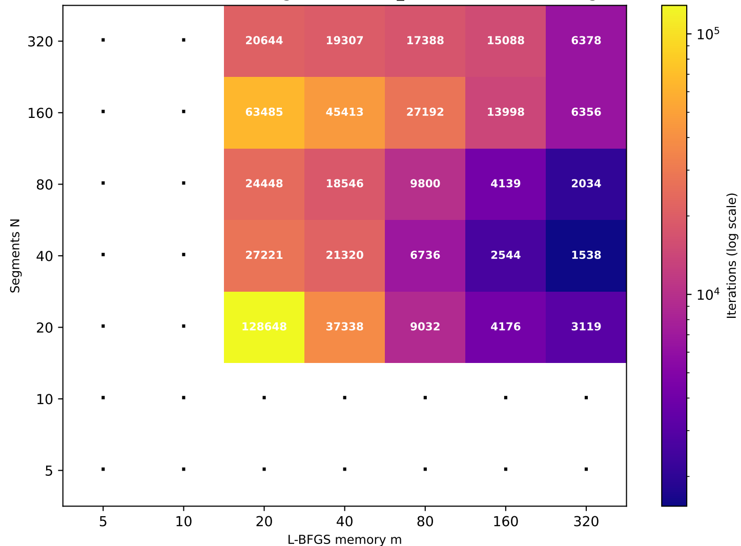
Recurrence T \approx 81.51 (target T=80 , rec_id=20) [25/49 converged]
