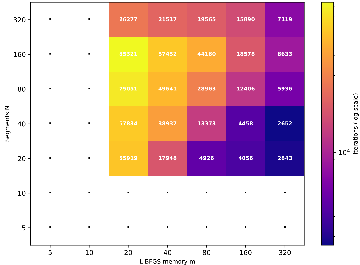
Recurrence T \approx 81.14 (target T=80 , rec_id=21) [25/49 converged]
