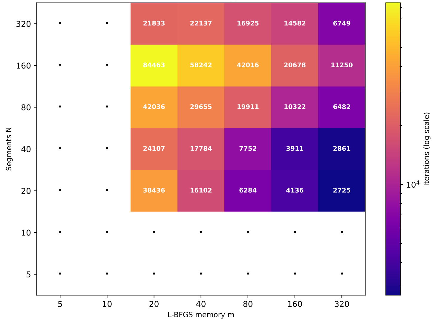
Recurrence T \approx 81.93 (target T=80 , rec_id=23) [25/49 converged]
