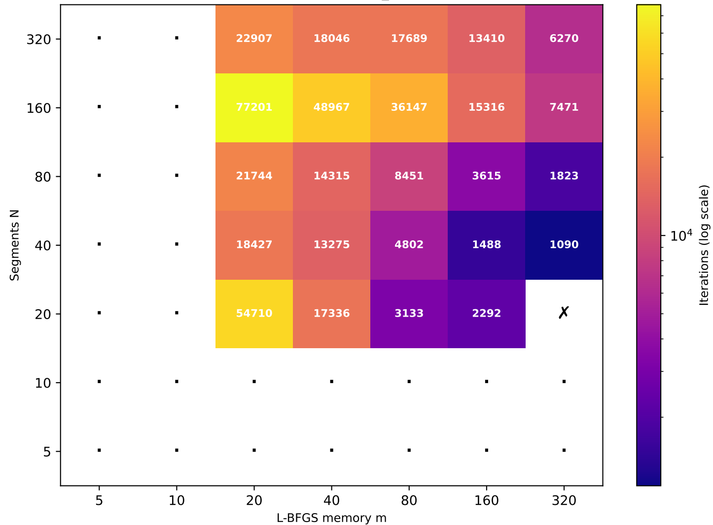
Recurrence T \approx 78.21 (target T=80 , rec_id=27) [24/49 converged]
