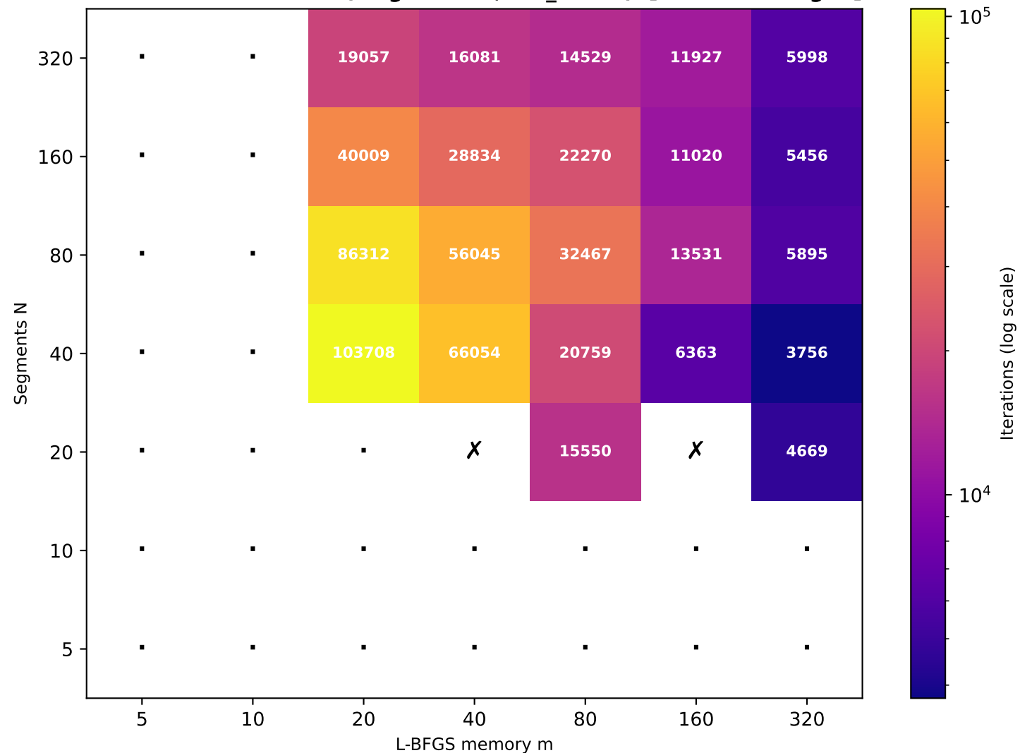
Recurrence T \approx 78.12 (target T=80 , rec_id=30) [22/49 converged]
