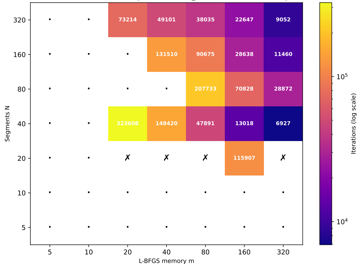
Recurrence T \approx 81.79 (target T=80 , rec_id=32) [18/49 converged]
