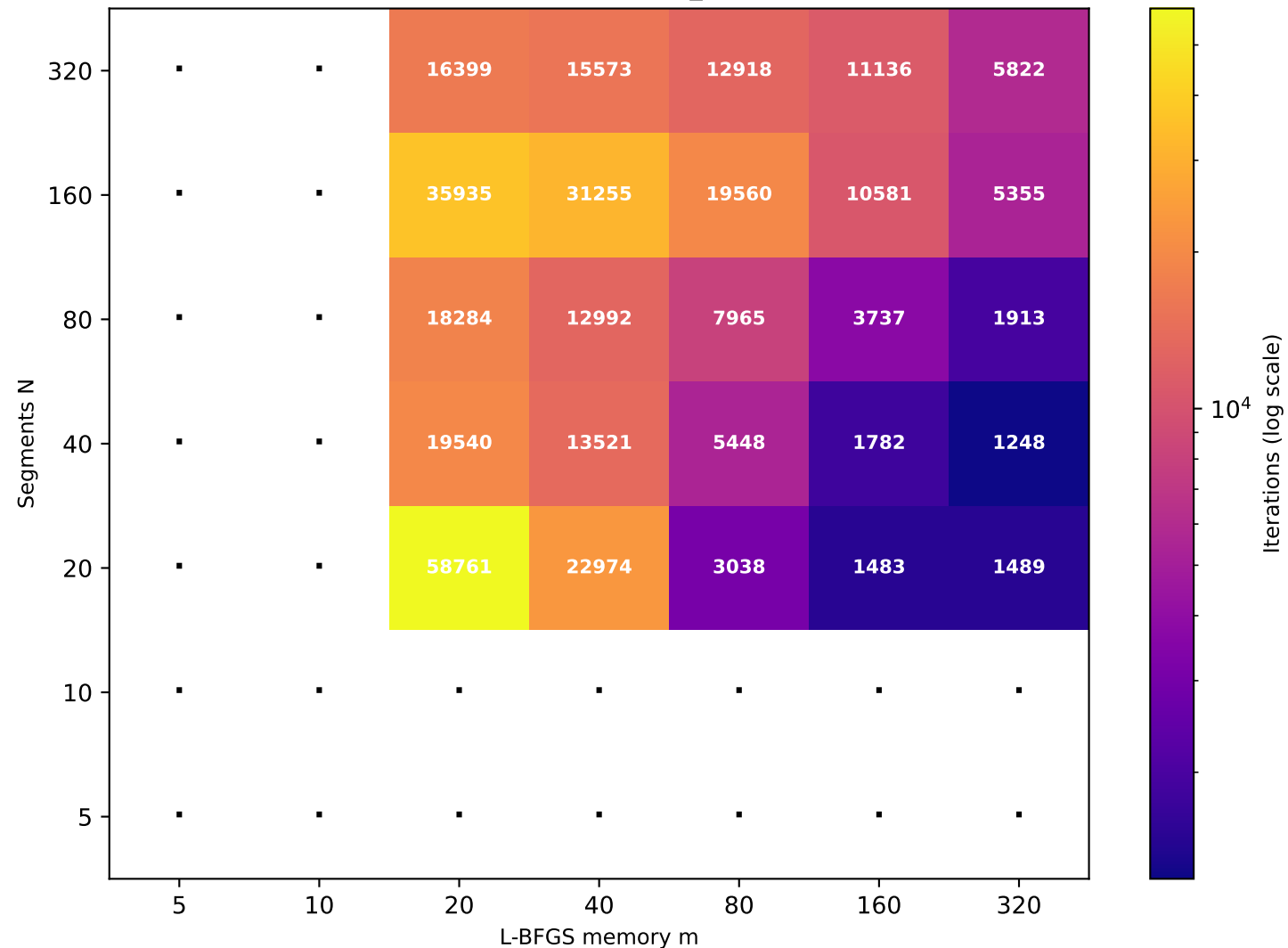
Recurrence T \approx 78.07 (target T=80 , rec_id=34) [25/49 converged]
