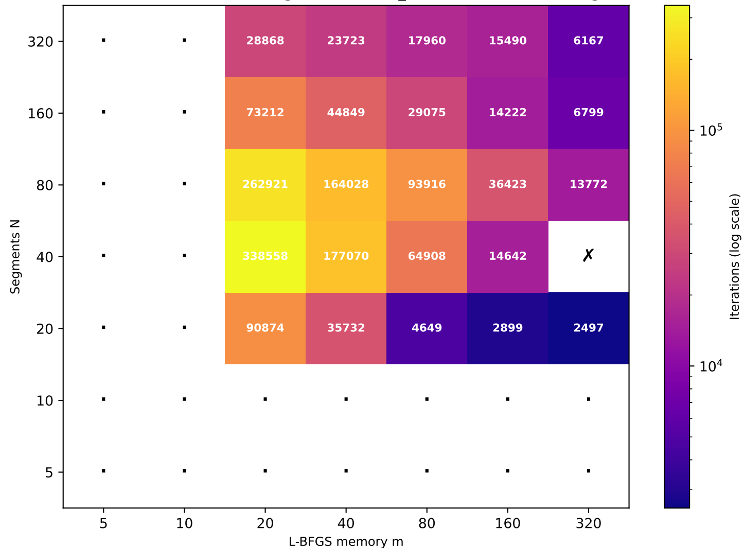
Recurrence T \approx 80.14 (target T=80 , rec_id=39) [24/49 converged]
