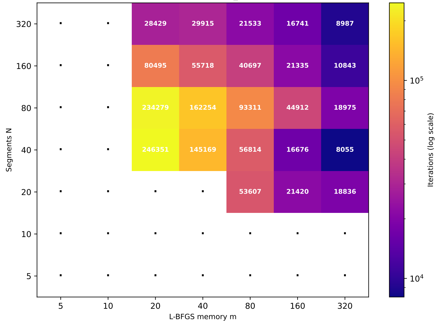
Recurrence T \approx 79.09 (target T=80 , rec_id=40) [23/49 converged]
