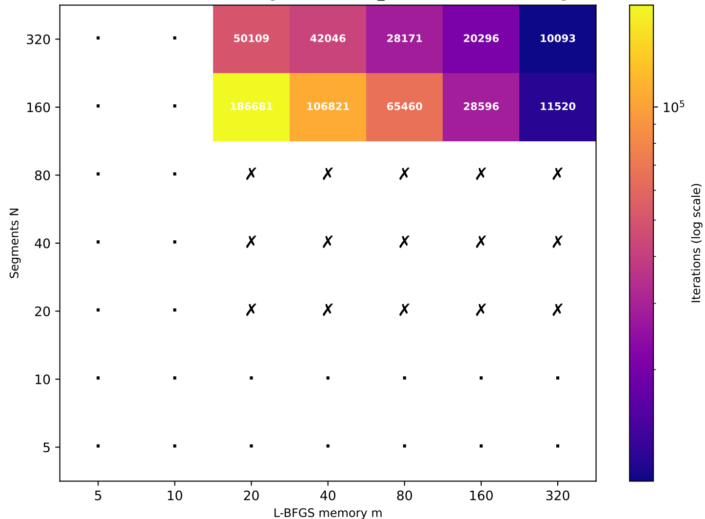
Recurrence T \approx 79.59 (target T=80 , rec_id=43) [10/49 converged]
