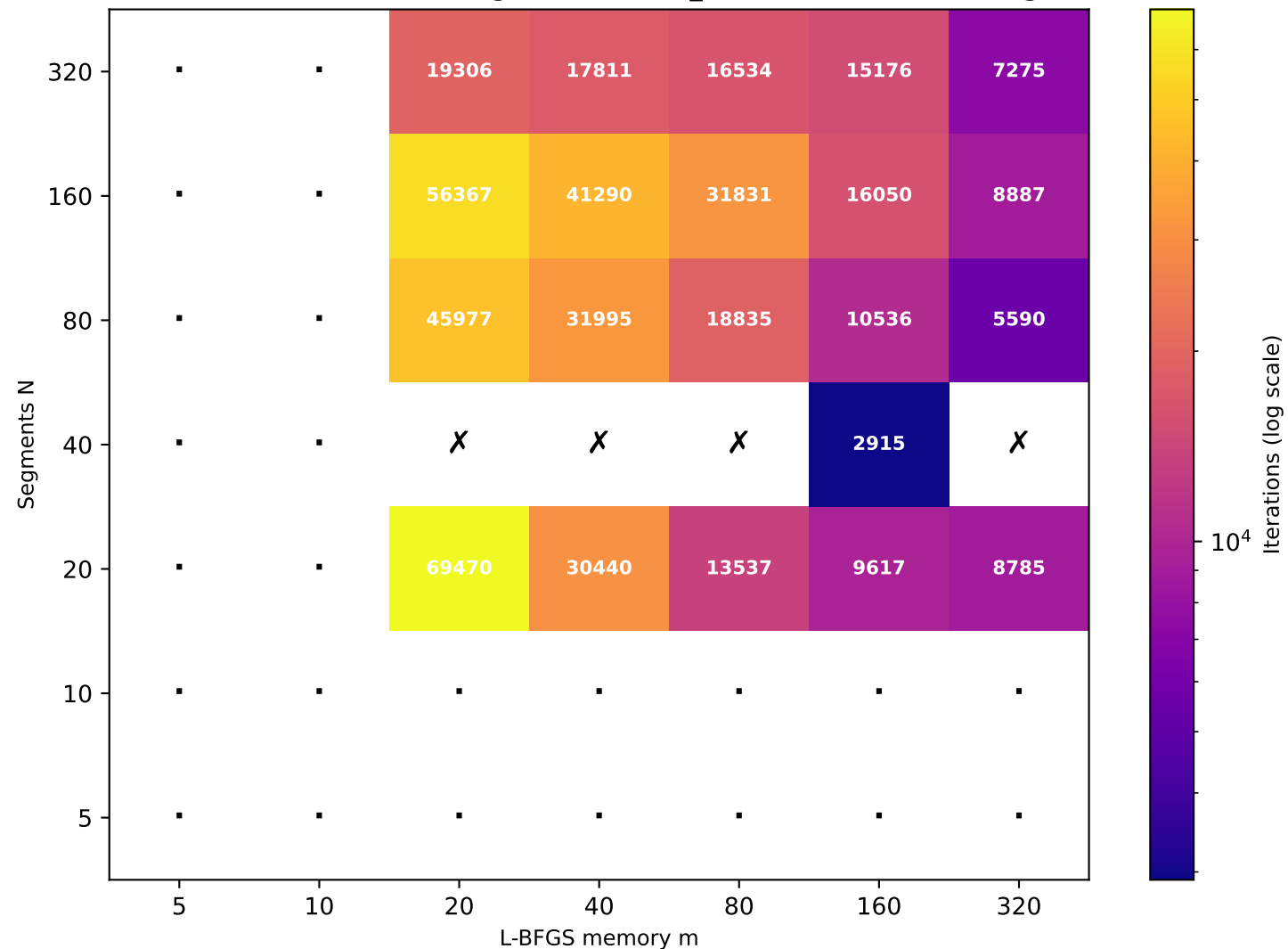
Recurrence T \approx 81.82 (target T=80 , rec_id=45) [21/49 converged]
