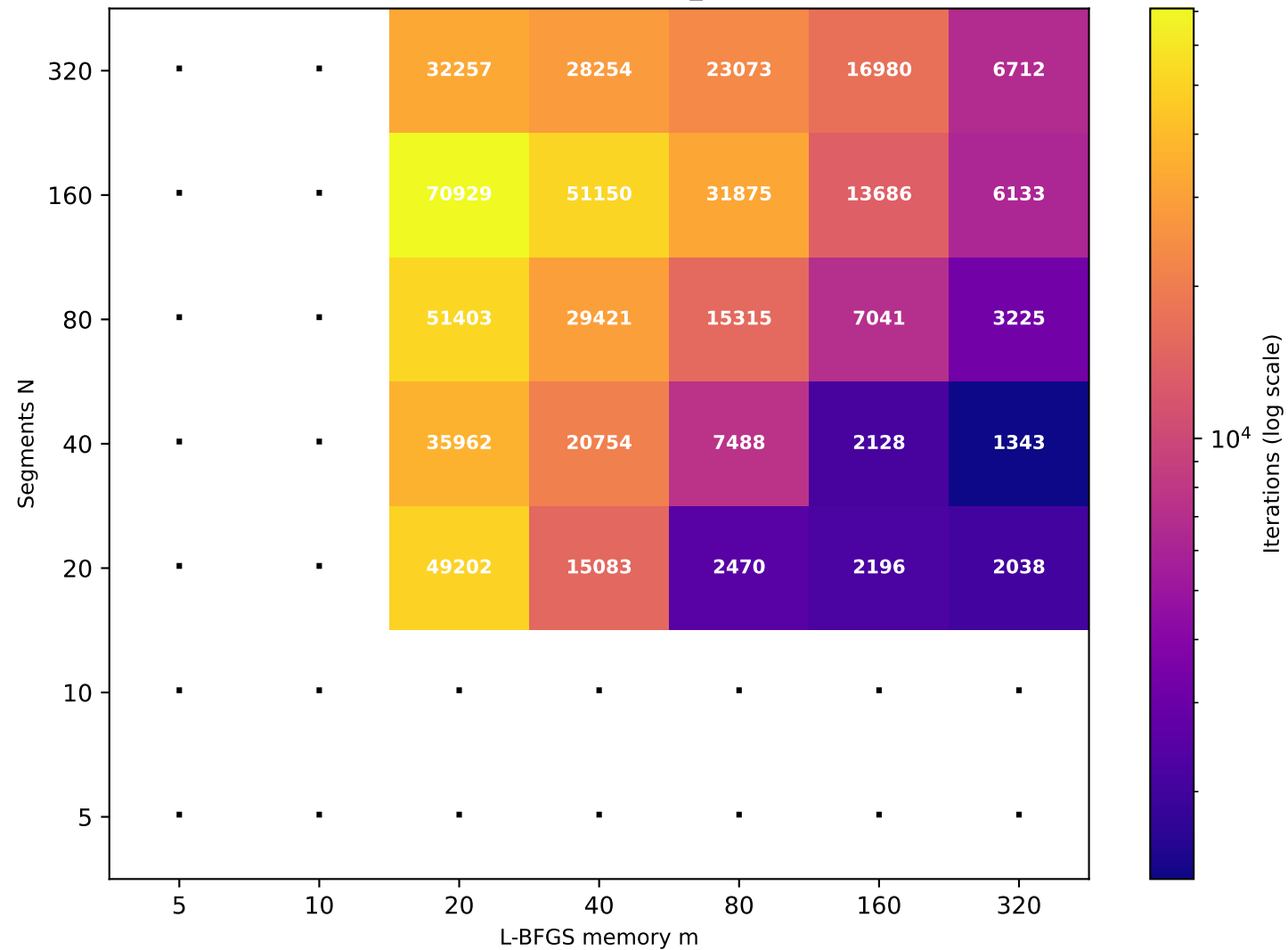
Recurrence T \approx 81.99 (target T=80 , rec_id=50) [25/49 converged]
