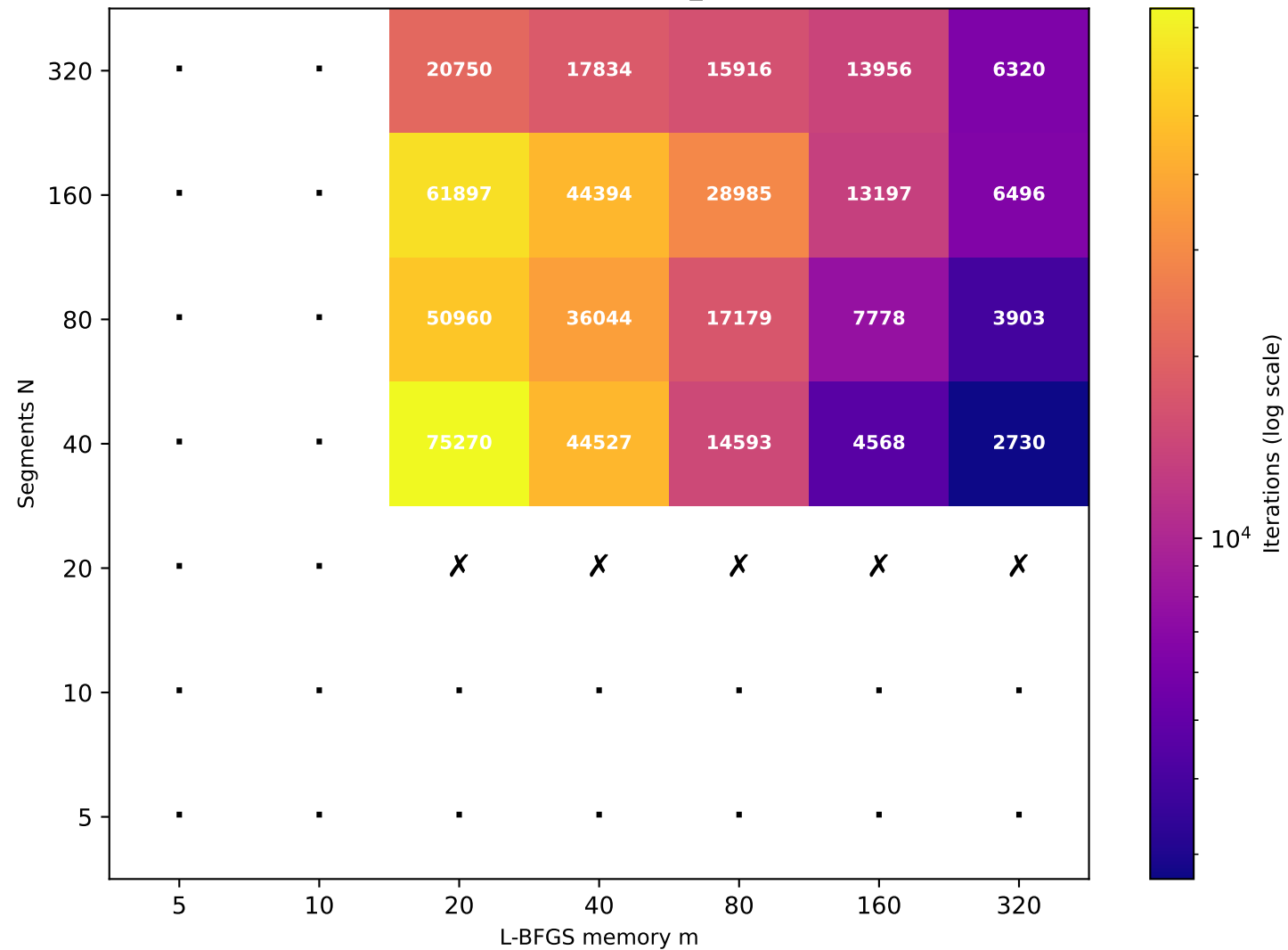
Recurrence T \approx 78.67 (target T=80 , rec_id=54) [20/49 converged]
