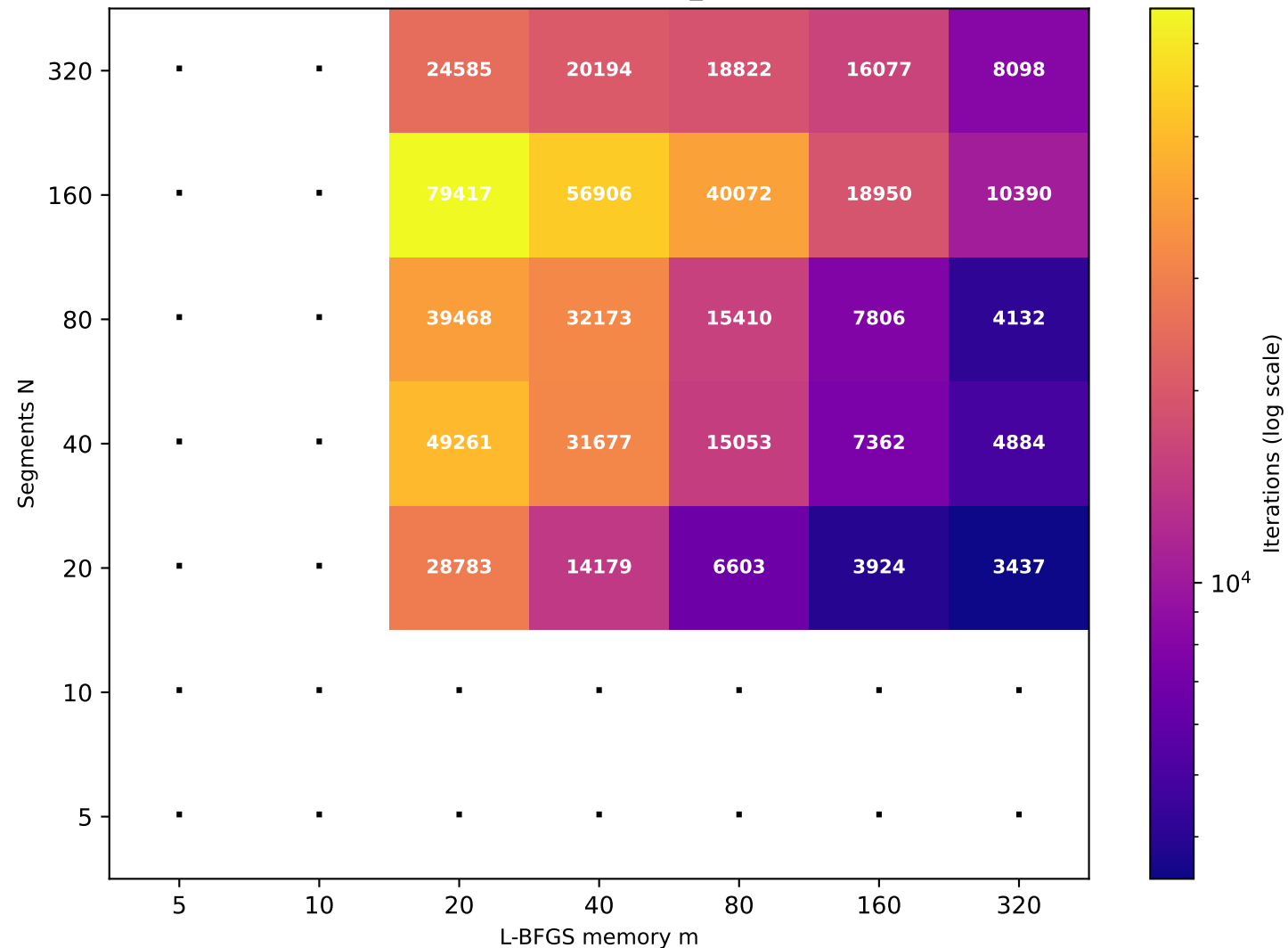
Recurrence T \approx 80.06 (target T=80 , rec_id=55) [25/49 converged]
