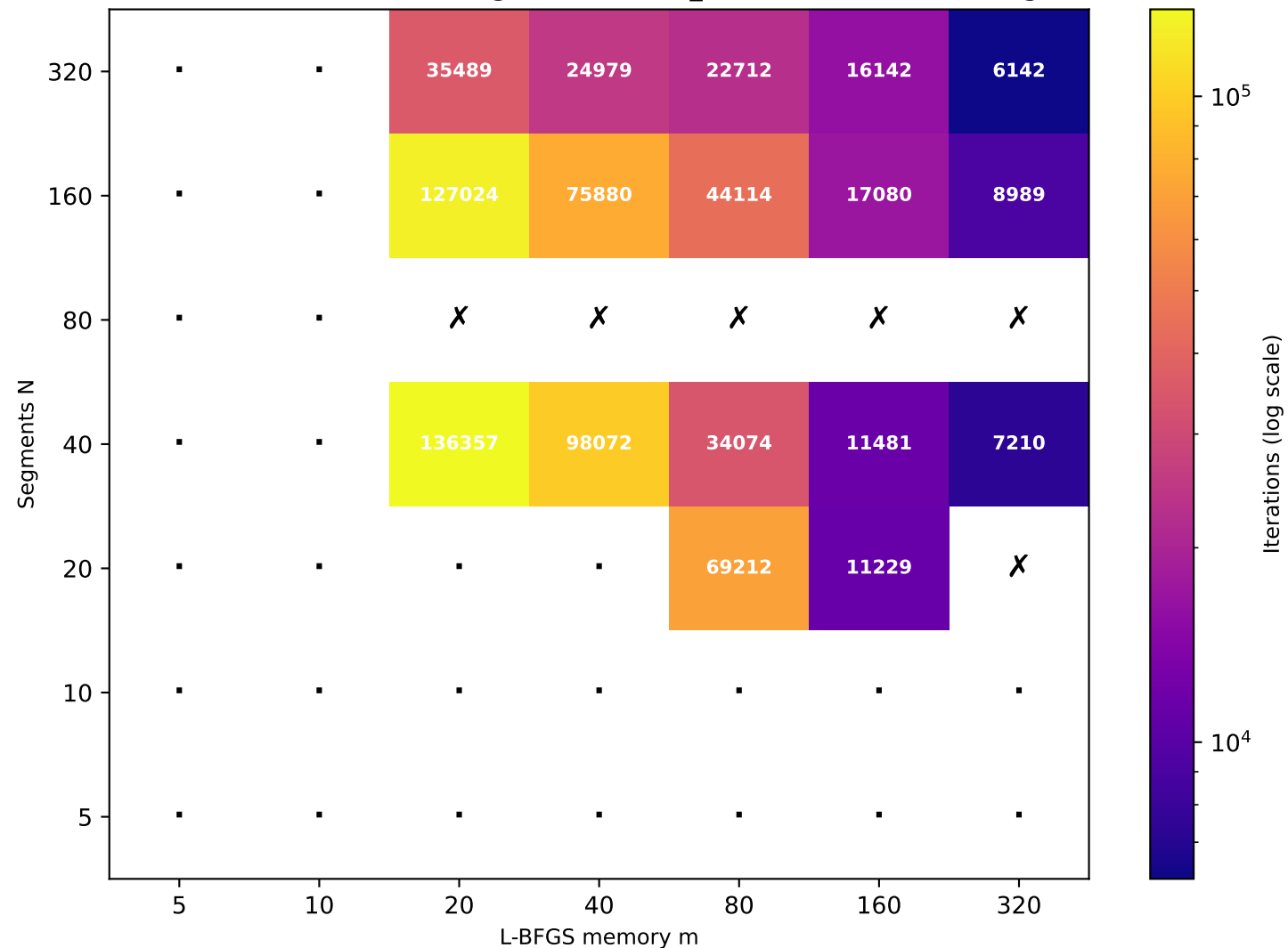
Recurrence T \approx 80.41 (target T=80 , rec_id=57) [17/49 converged]
