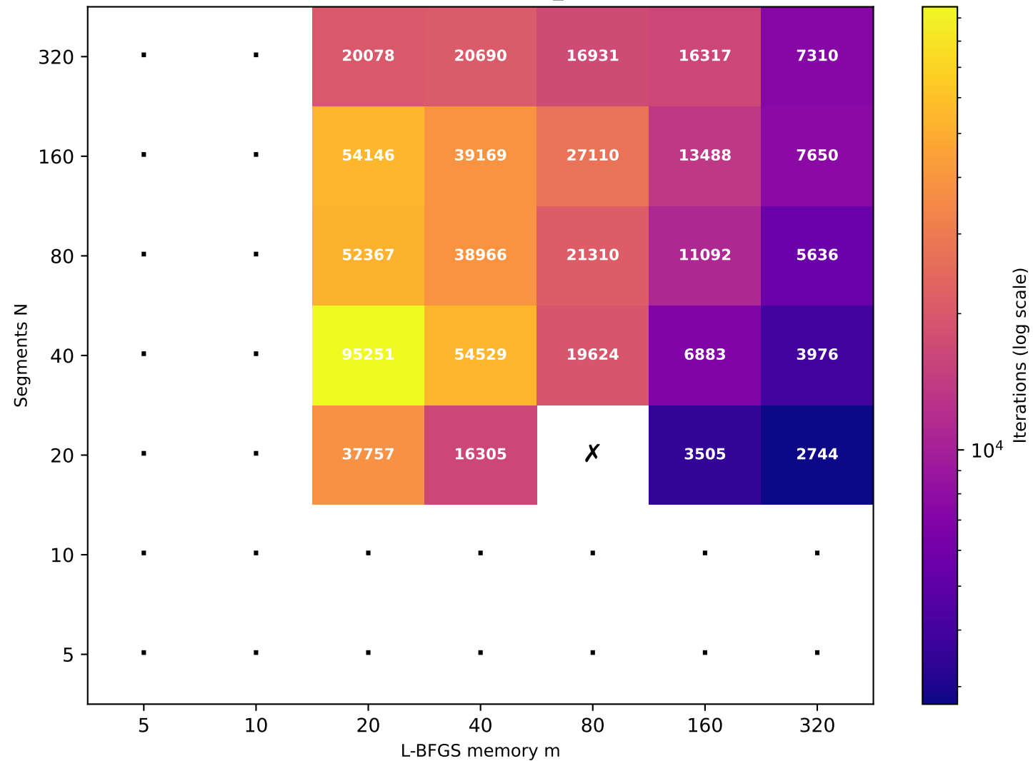
Recurrence T \approx 80.60 (target T=80 , rec_id=58) [24/49 converged]
