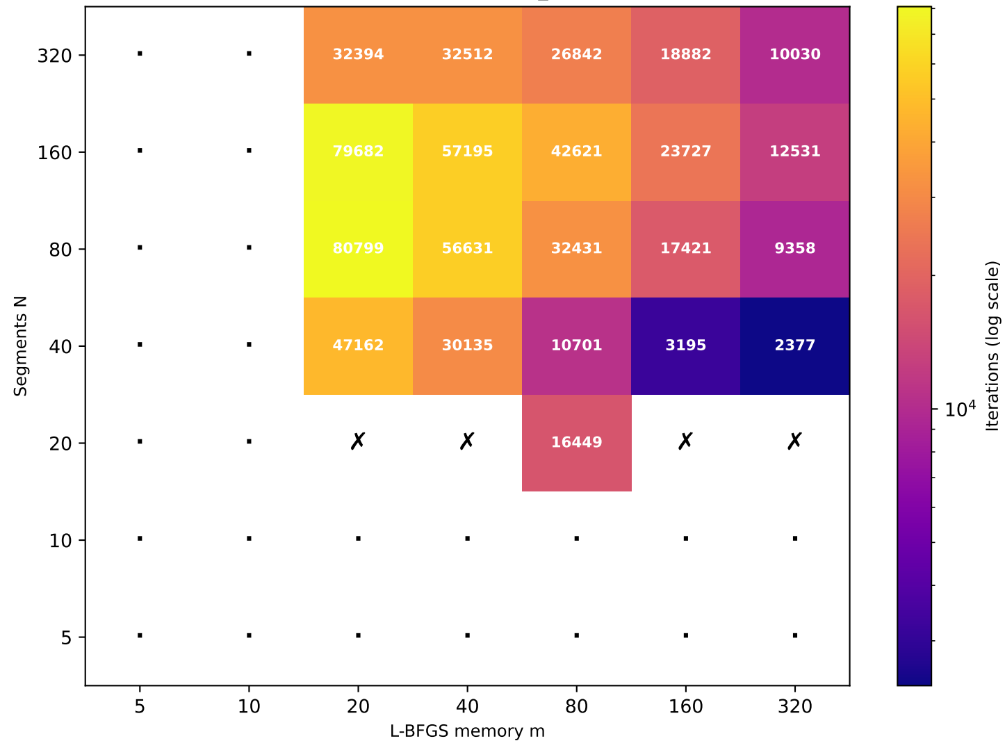
Recurrence T \approx 79.76 (target T=80 , rec_id=60) [21/49 converged]
