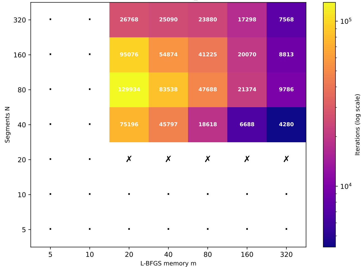
Recurrence T \approx 78.14 (target T=80 , rec_id=61) [20/49 converged]
