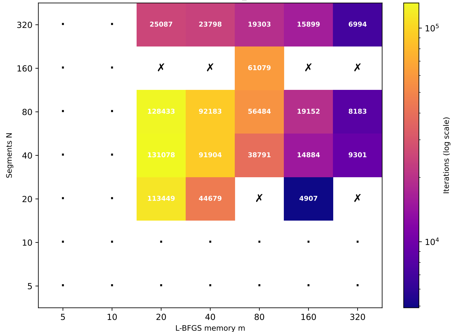
Recurrence T \approx 81.47 (target T=80 , rec_id=62) [19/49 converged]
