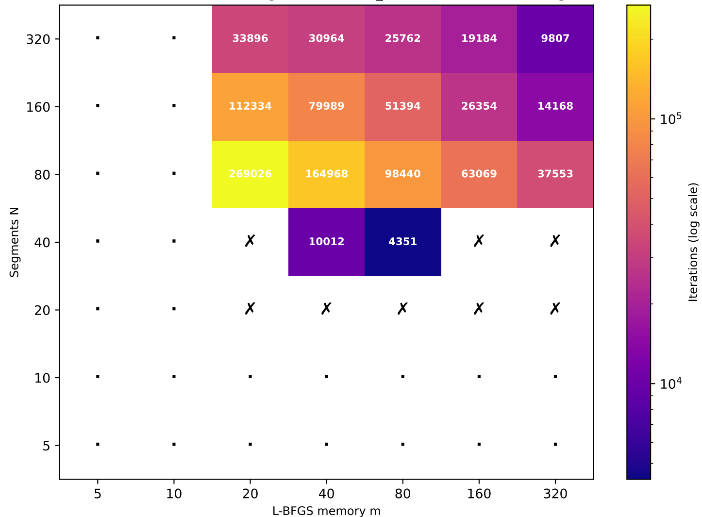
Recurrence T \approx 79.84 (target T=80 , rec_id=64) [17/49 converged]
