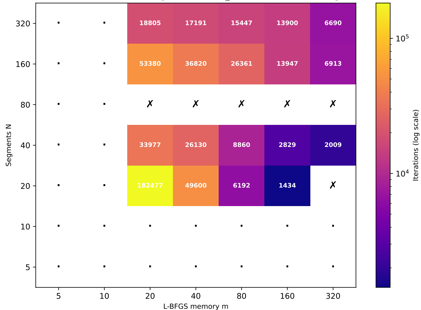
Recurrence T \approx 79.22 (target T=80 , rec_id=67) [19/49 converged]
