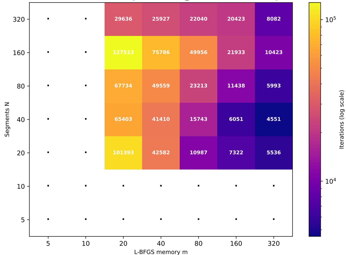
Recurrence T \approx 81.80 (target T=80 , rec_id=69) [25/49 converged]
