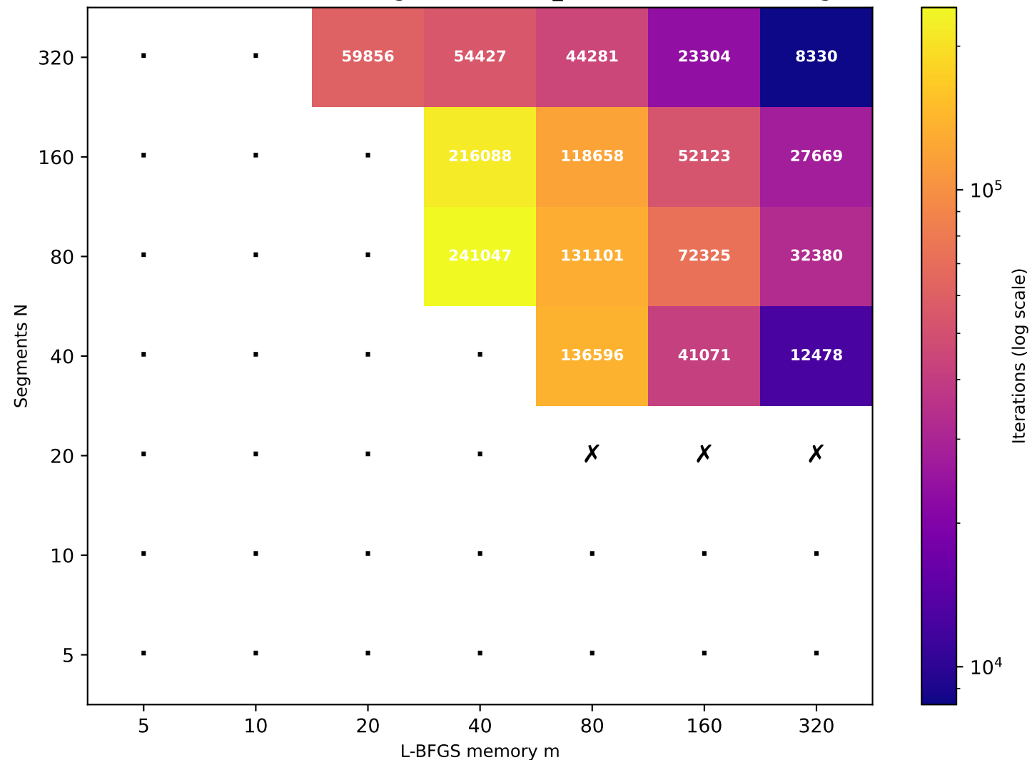
Recurrence T \approx 80.75 (target T=80 , rec_id=71) [16/49 converged]
