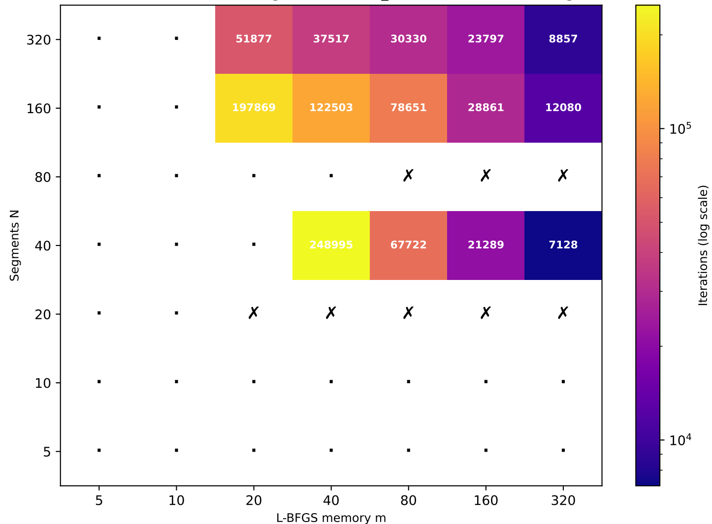
Recurrence T \approx 77.81 (target T=80 , rec_id=72) [14/49 converged]
