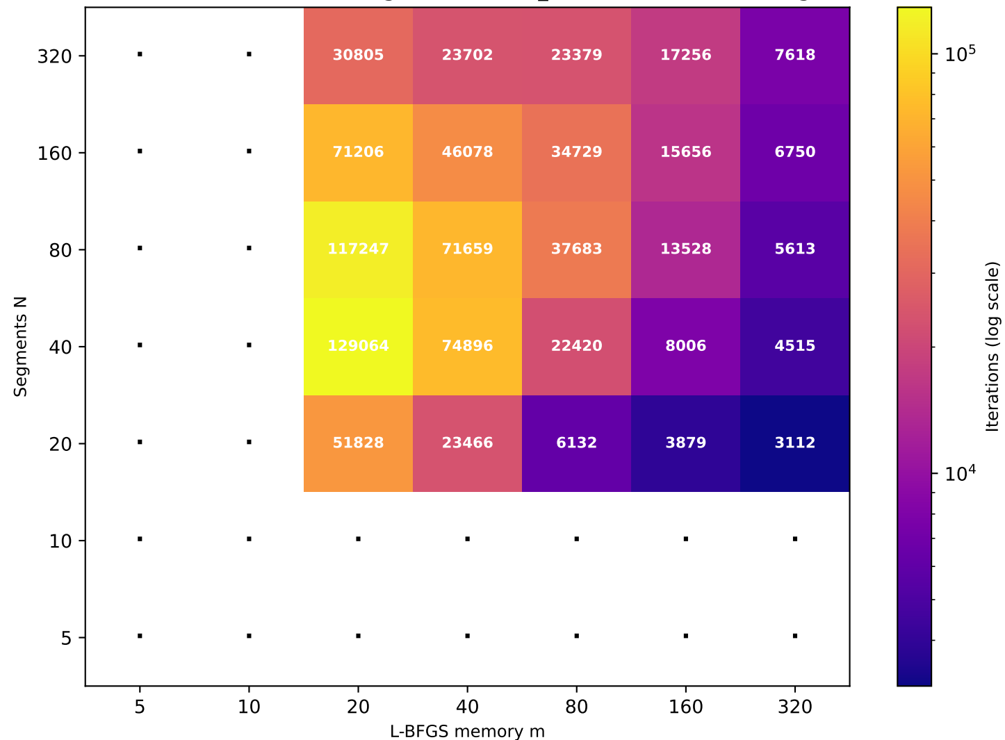
Recurrence T \approx 80.80 (target T=80 , rec_id=73) [25/49 converged]
