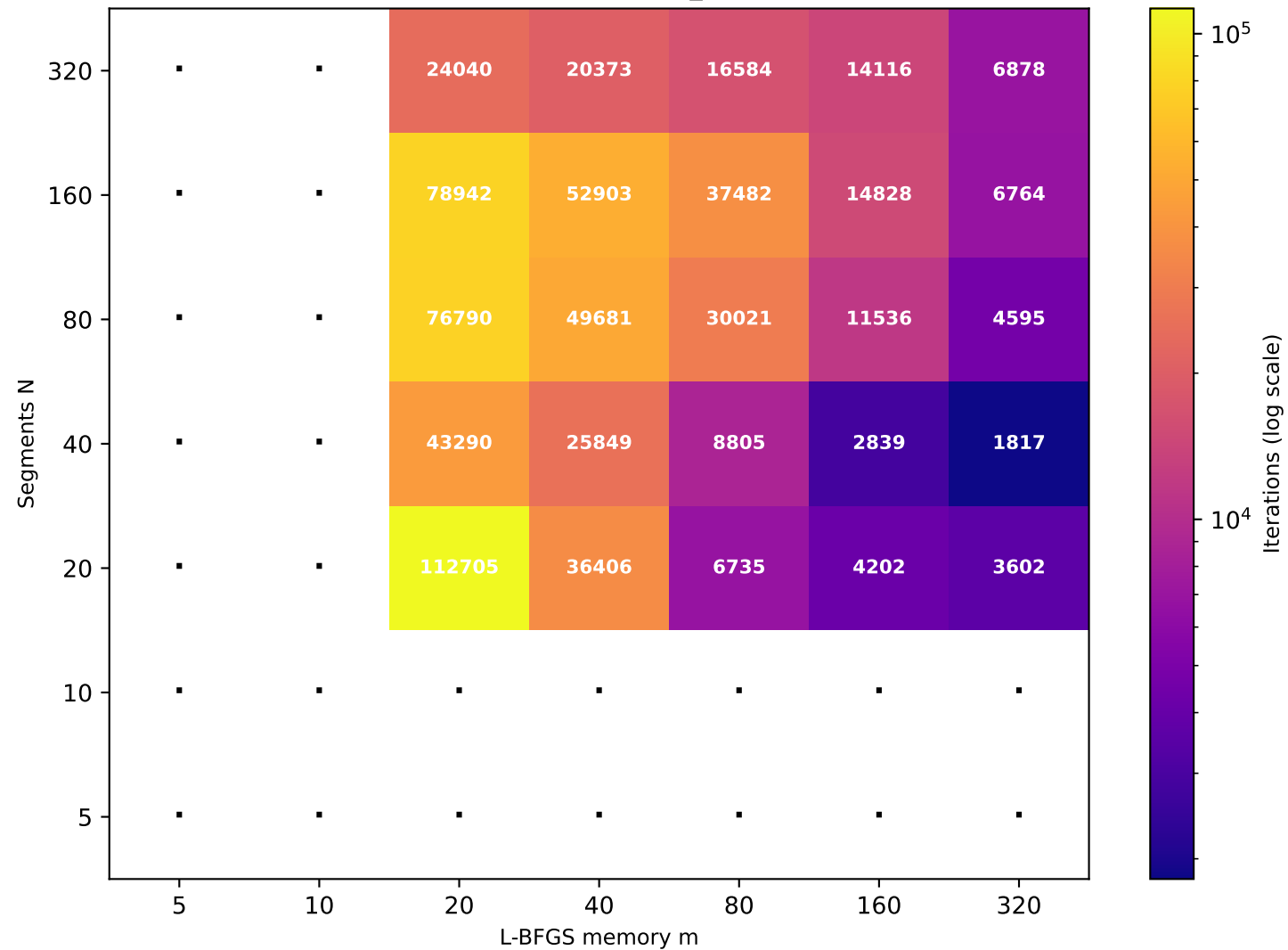
Recurrence T \approx 80.30 (target T=80 , rec_id=75) [25/49 converged]
