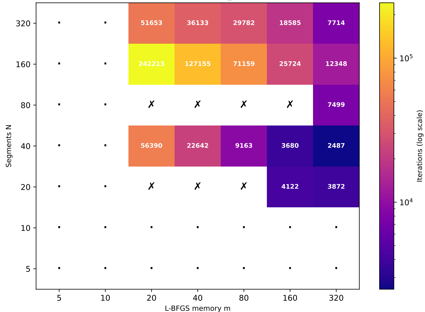
Recurrence T \approx 77.90 (target T=80 , rec_id=76) [18/49 converged]
