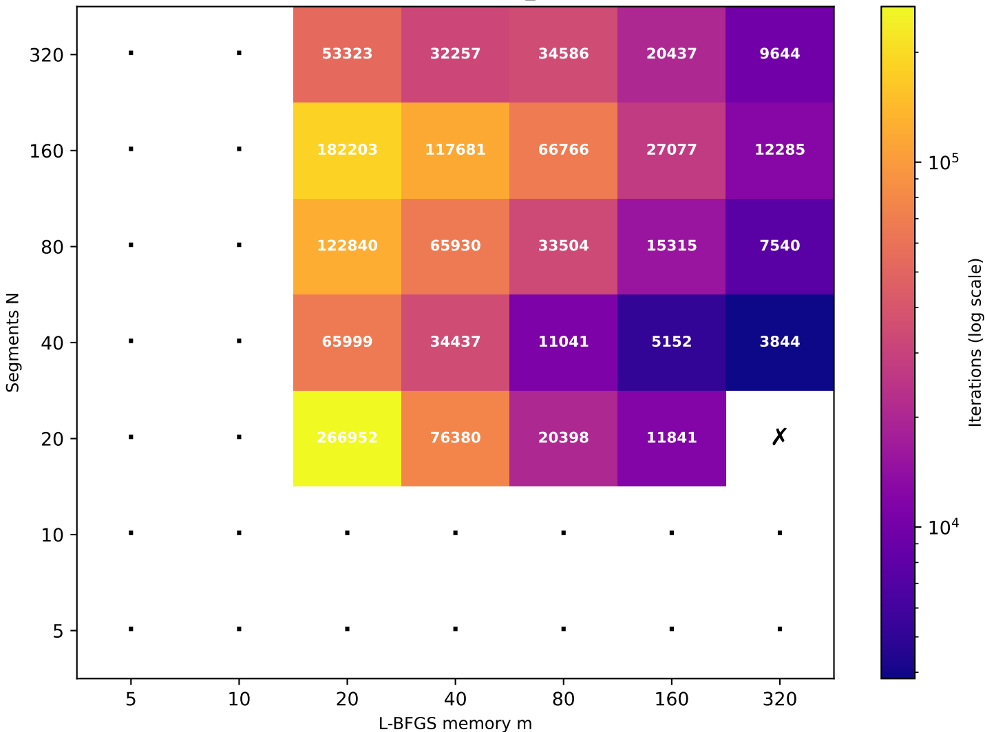
Recurrence T \approx 81.11 (target T=80 , rec_id=80) [24/49 converged]
