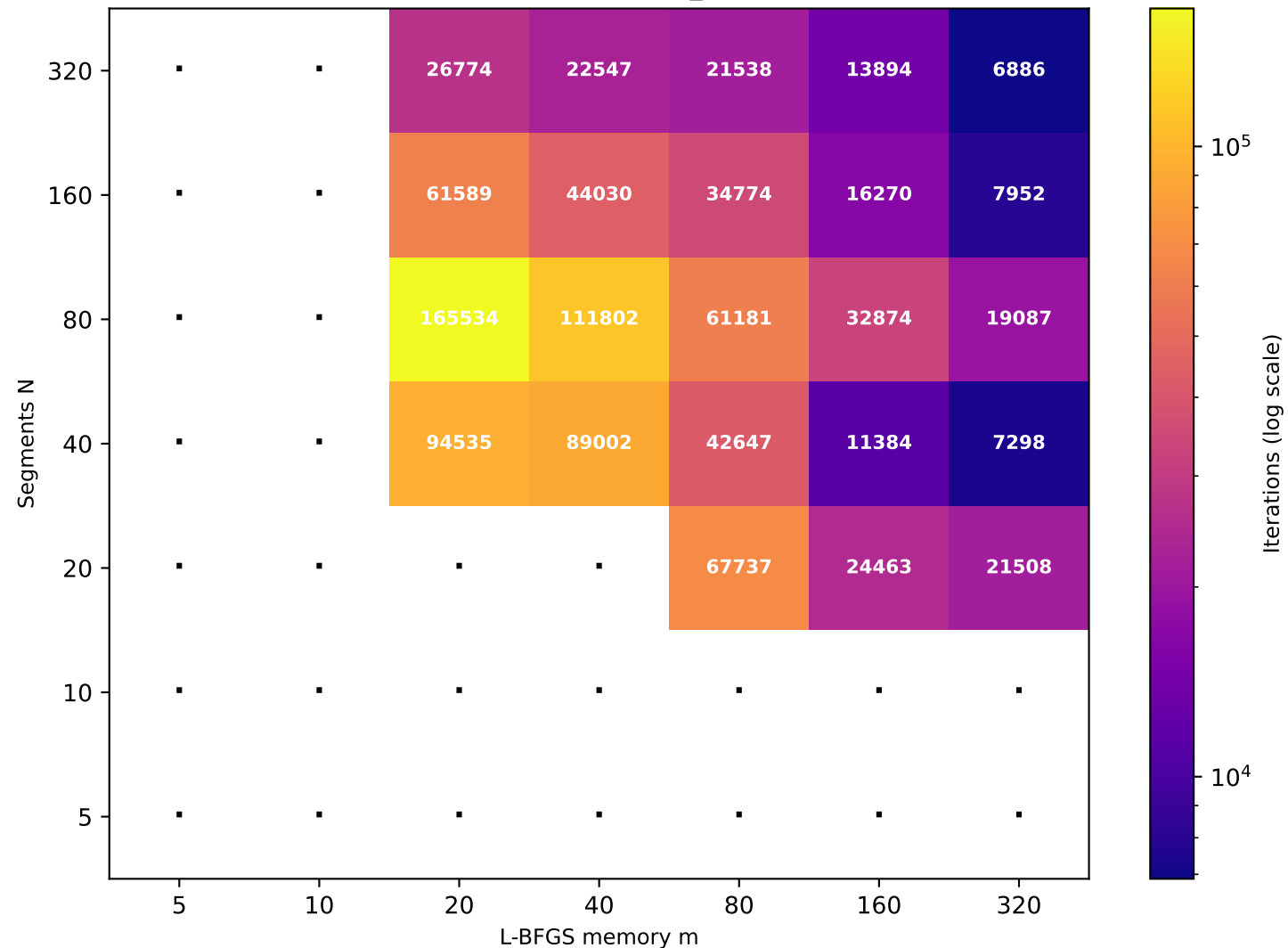
Recurrence T \approx 78.95 (target T=80 , rec_id=82) [23/49 converged]
