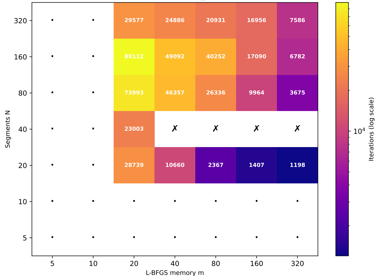
Recurrence T \approx 80.76 (target T=80 , rec_id=87) [21/49 converged]
