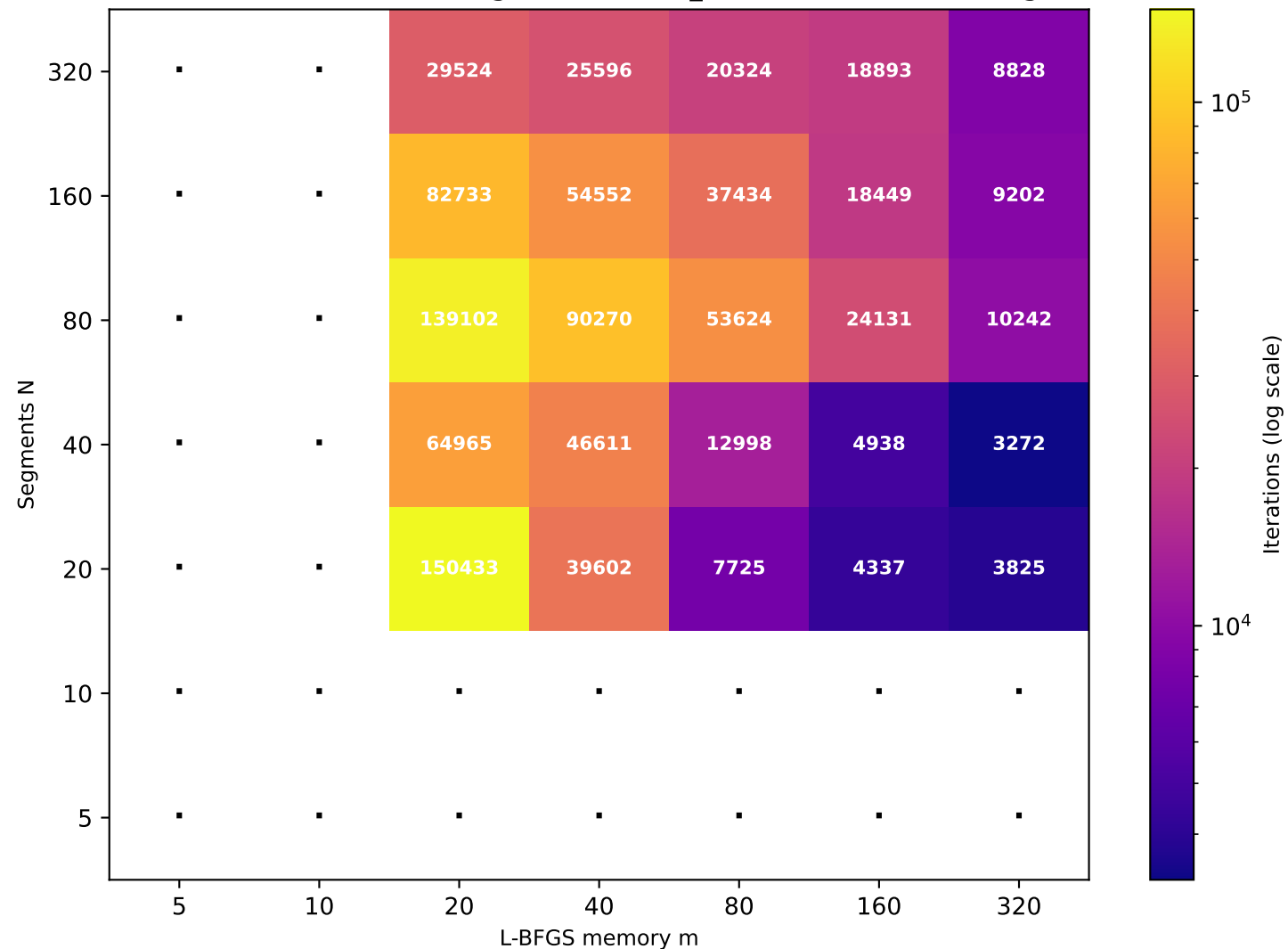
Recurrence T \approx 81.61 (target T=80 , rec_id=88) [25/49 converged]
